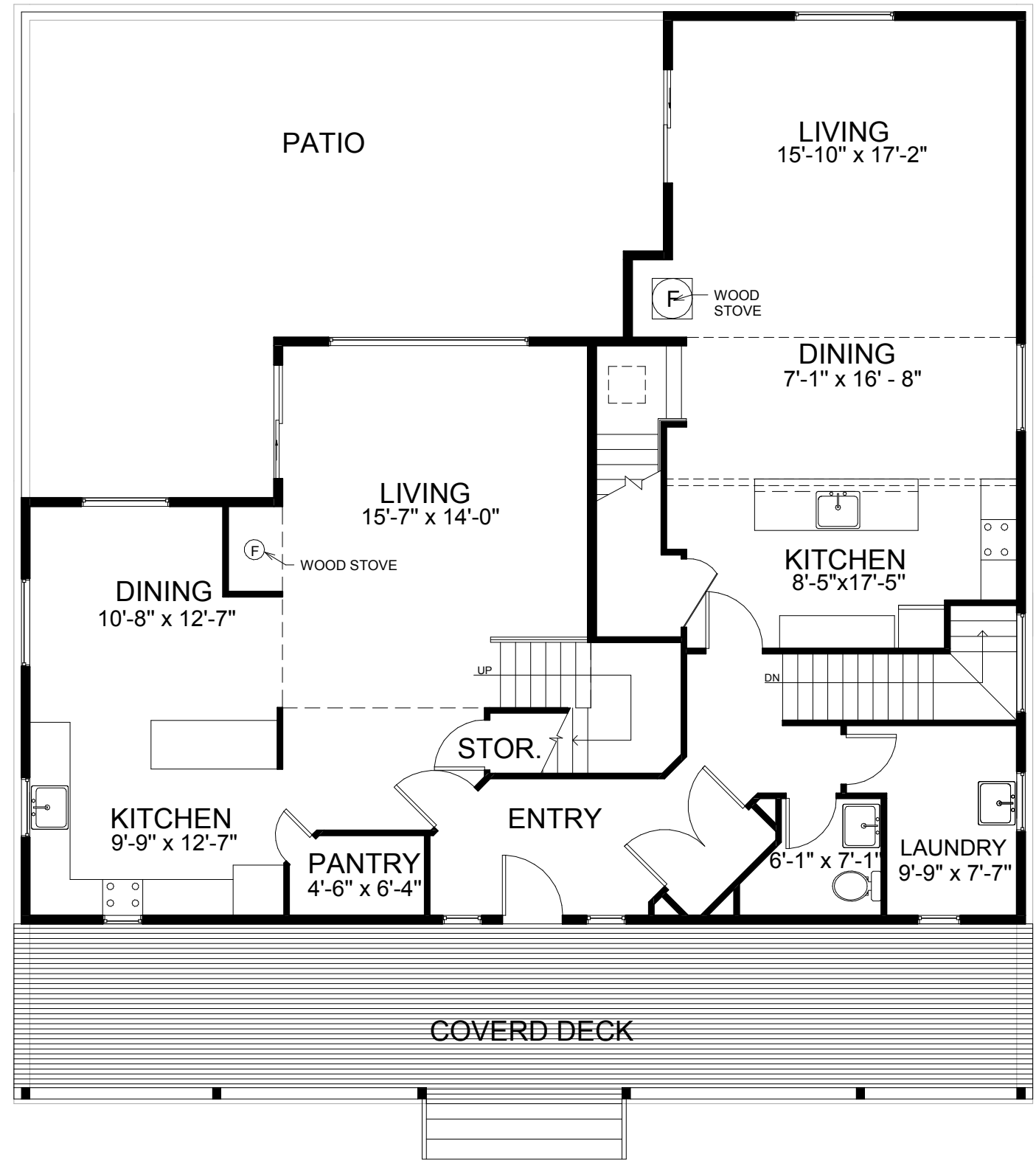
CARETAKER COTTAGE - LEVEL 2
