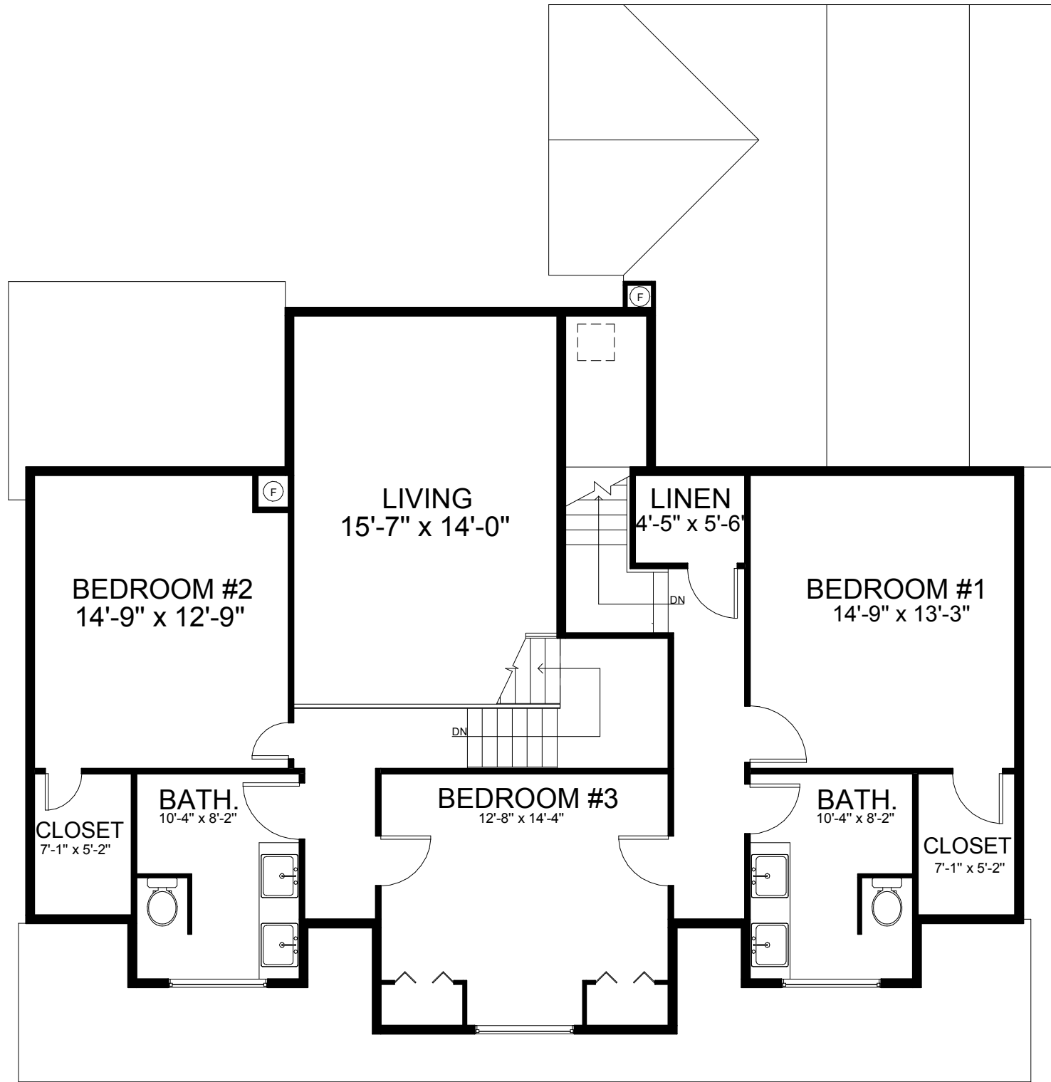
CARETAKER COTTAGE - LEVEL 3
