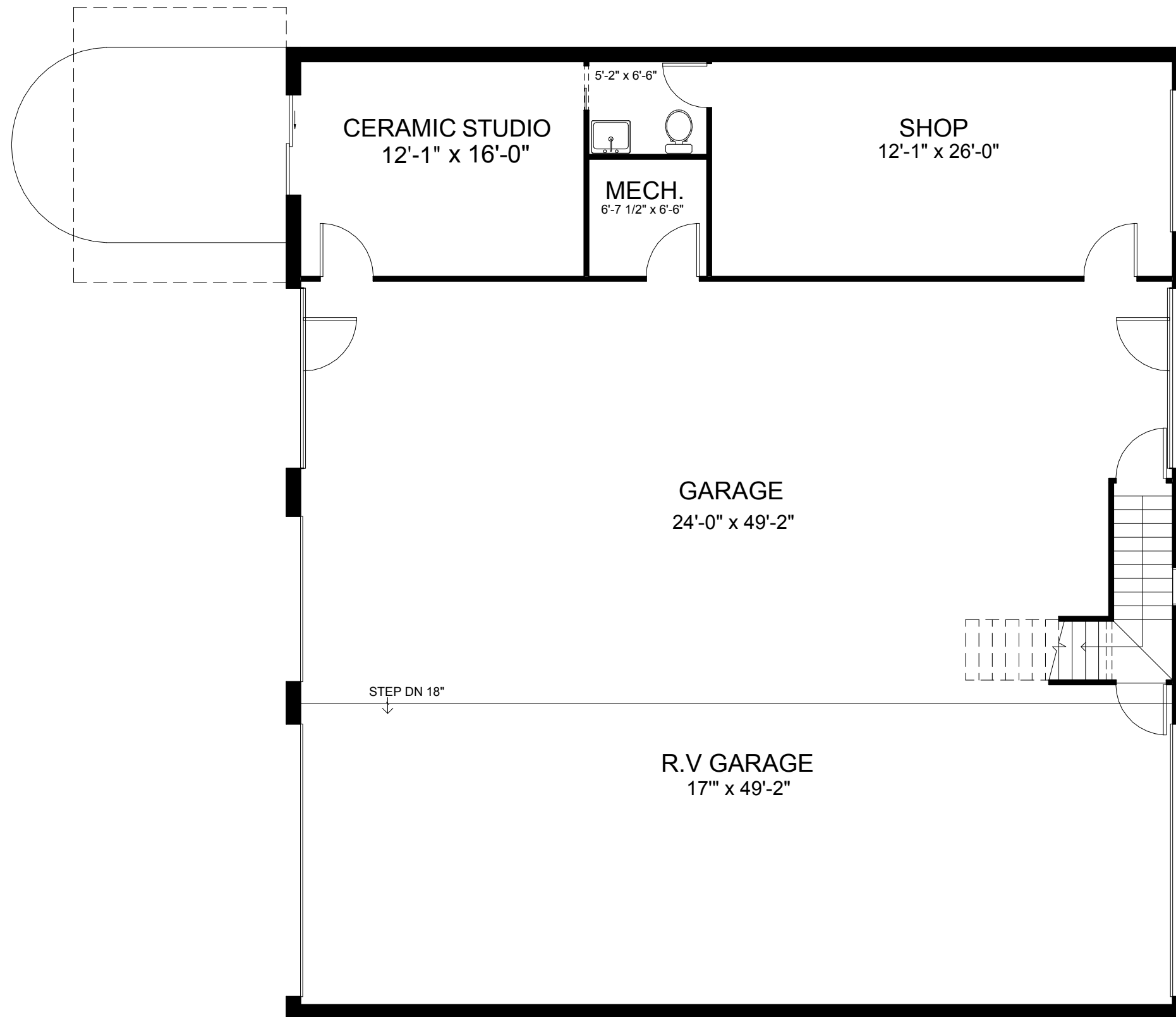
CARETAKER COTTAGE - LEVEL 1
