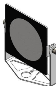
Fig. 5: LaserTilt90 mounted on a swivel mounting bracket LS-ACC-LAS-SB that includes the attachment option of a convergence bolt with a G3/8" male thread.
