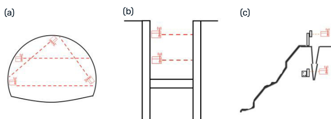
Fig. 1: Different applications for the LaserTil90. (a) convergence monitoring in tunnels and galleries, (b) convergence monitoring in construction shaft, (c) crack monitoring in open pit mines and rock slopes.
