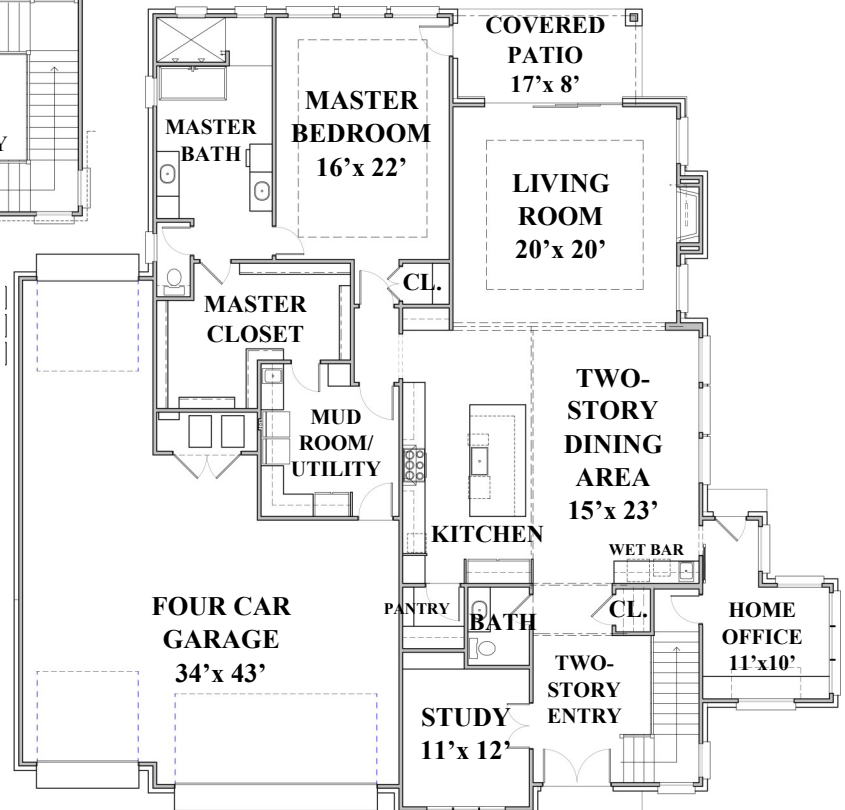
LOWER FLOOR
