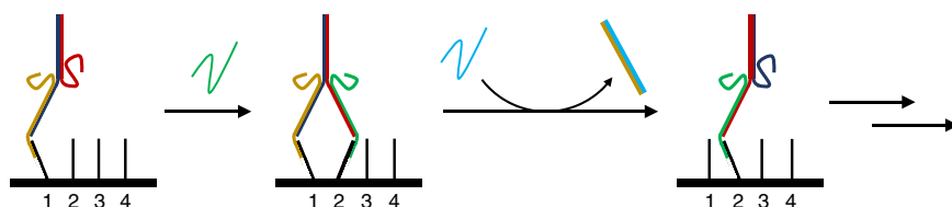
Figure 14.10 Programmed motion of a bipedal DNA walker. An attaching strand (in green) connects the second leg of the walker. Subsequently, a strand displacement reaction can occur that sees the attaching strand connecting the first leg (in gold) to the track being displaced by a detaching strand (in light blue). This way, the walker has moved from station 1 to station 2. Walking toward station 4 was achieved following the same stepwise mechanism.
