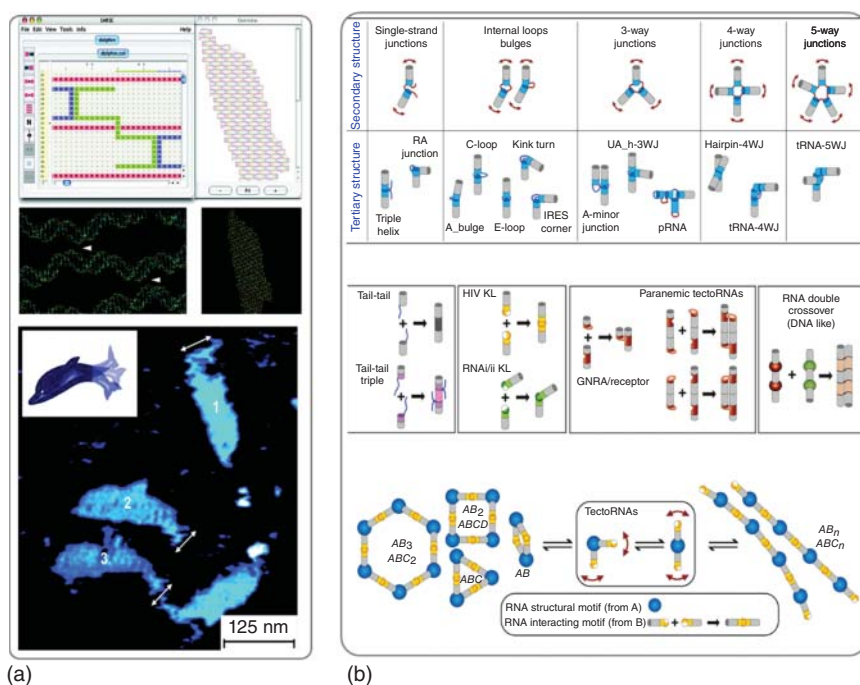
Figure 5.1 Nucleic acid nanostructure designing techniques. (a) DNA origami method was used to computationally design and assemble a dolphin-shaped DNA nanostructure. (b) Example of RNA nanoparticle design approach. Variety of RNA tertiary structures (tecto-RNAs) were combined to construct different nano-objects of 1D or linear shape, 2D or polygonal shapes, and 3D shapes. Source: (Panel a) From Andersen et al. [27]. Reprinted with the permission of American Chemical Society; (Panel b) From Grabow and Jaeger [28]. Reproduced with the permission of American Chemical Society.
