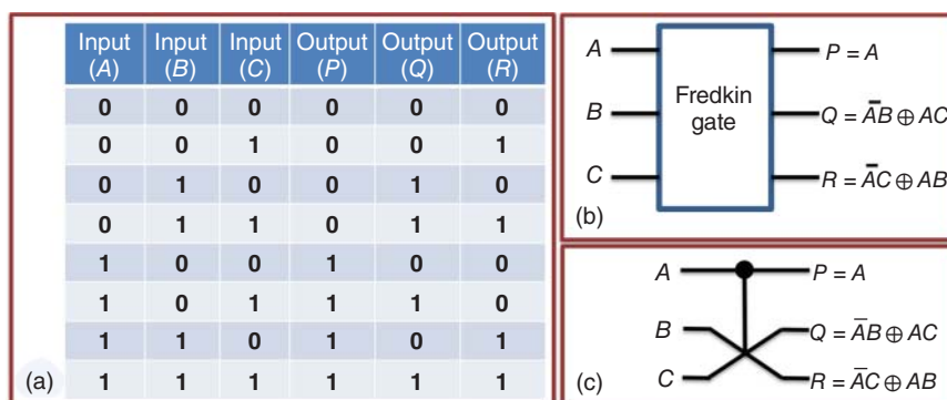
Figure 19.8 The truth table (a), block diagram (b), and equivalent electronic circuitry (c) for the Fredkin gate. Standard Boolean notations are used in the schemes [82]. Source: From Fratto and Katz [71]. Reproduced with the permission of John Wiley & Sons.
