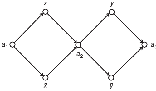
Figure 14.15 Graphical representation of a 2-SAT problem.
