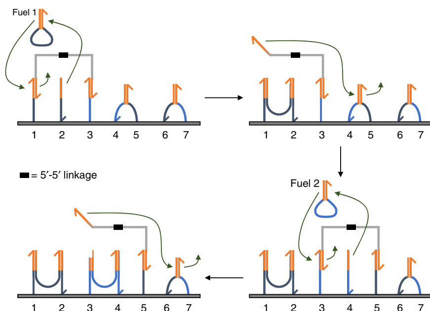
Figure 14.11 Autonomous directional motion of a DNA bipedal walking device. The movement of one leg from one station to the next is achieved by hybridization of a metastable DNA fuel strand that displaces the leg from its station. The leg can subsequently bind the next station by strand displacement reaction.
