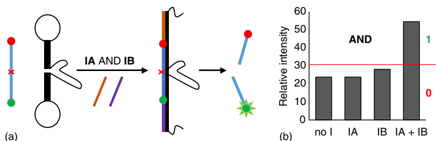
Figure 14.17 (a) Deoxyribozyme-based AND logic gate design with hairpins present at both ends of the gate strand. According to the Boolean truth table, the addition of both inputs will result in the opening of the two hairpins, allowing the fluorescent strand to hybridize. The latter is subsequently cleaved leading to fluorescence emission. (b) Relative fluorescence observed depending on the input added to the system. Only the addition of both inputs induces a characteristic increase in the fluorescence emission.
