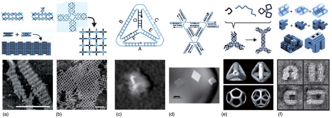
Figure 6.1 Representative tile-based DNA nanostructures. (a) 2D DNA crystalline arrays self-assembled from synthetic DNA double-crossover tiles [9]. (b) 2D square lattice assembled with 4 \times 4 DNA tiles [10]. (c) DNA tetrahedral structure [11]. (d) Self-assembled 3D DNA crystal from a tensegrity DNA triangle motif [12]. (e) Hierarchical polyhedral DNA structures [13]. (f) 3D structures built with single-stranded tile DNA bricks [14].
