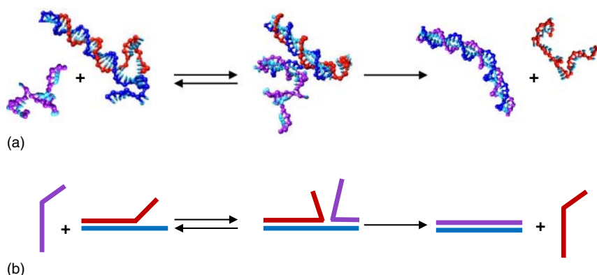
Figure 14.1 A prototypical DNA strand displacement reaction showing one of the ensembles of dynamic “walking” intermediates depicted using (a) OxDNA [2] coarse-grained modeling and (b) in simplified schematic form.
