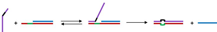
Figure 14.5 Remote toehold mechanism. A spacer separates the toehold and the branch migration domains. Modulation of the nature and size of the spacer allows to finely tune the kinetics of the strand displacement reaction.
