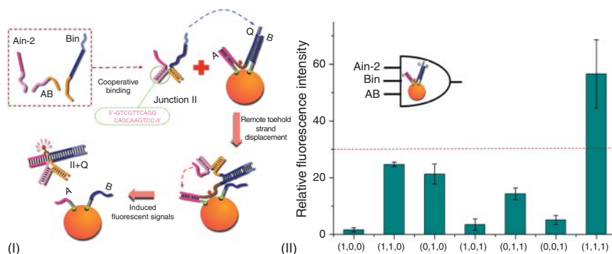
Figure 9.5 Three-input logic gate with an AuNP quencher. (I) Cooperative binding of inputs leading to remote toehold-mediated strand displacement and fluorescence restoration. (II) Fluorescent response of the three-input AND gate. Source: From Yang et al. [94]. Reproduced with the permission of American Chemical Society.
