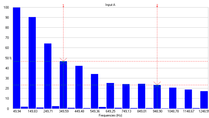
Figure 4 The Fourier spectrum of the wave shape in Fig 1. Note the high 150 Hz component.
