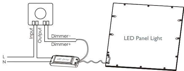
2 1-10V dimming version
