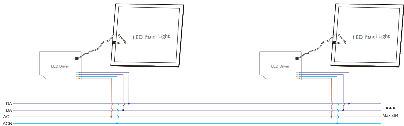
3 DALI dimming version
