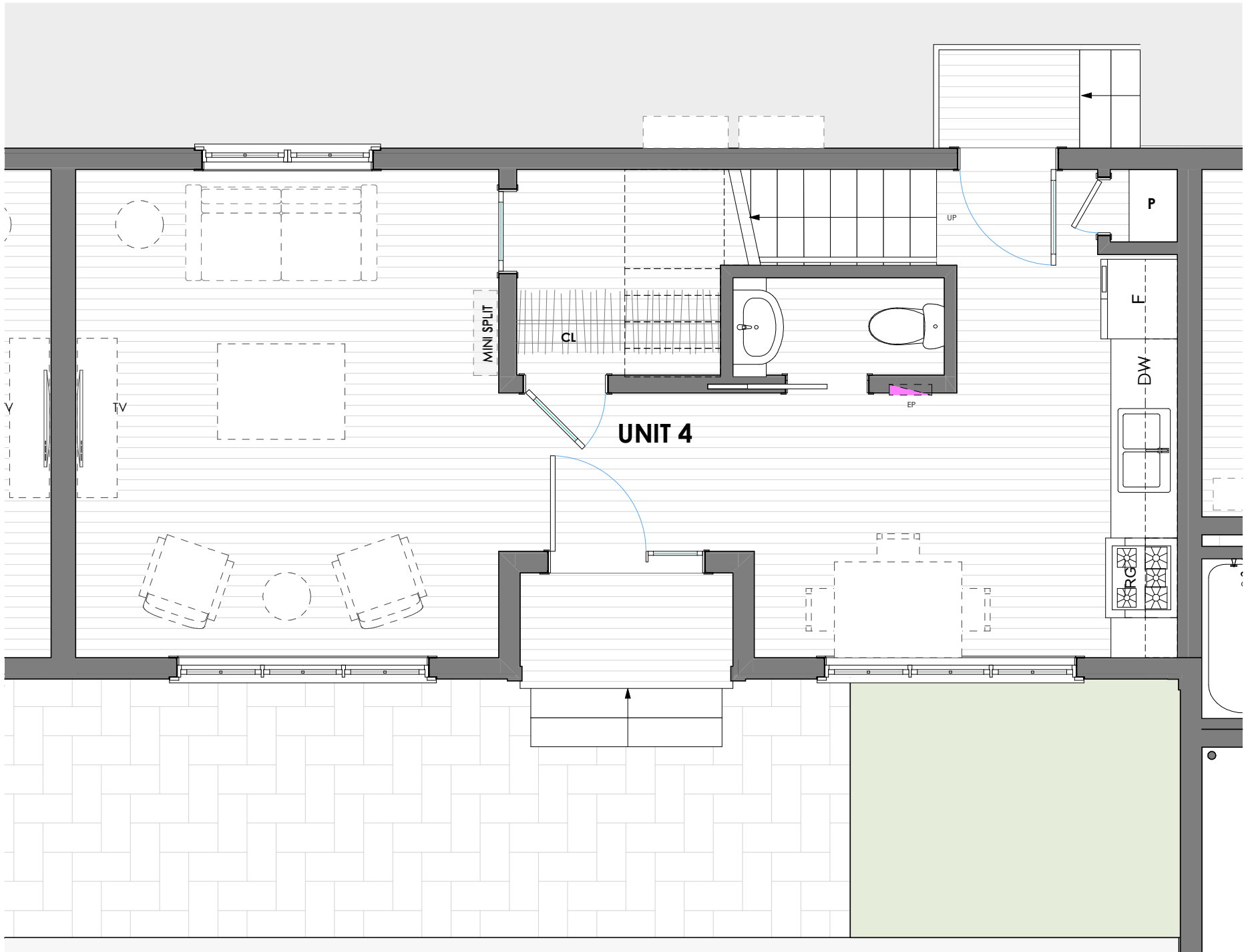
1 UNIT 4 -1ST FLOOR 1/4" = 1'-0"
