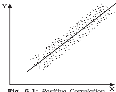
Fig. 6.1: Positive Correlation
