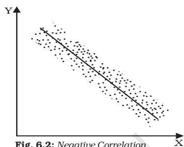
Fig. 6.2: Negative Correlation
