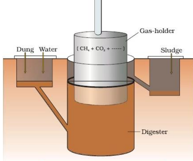
Fig.4. Gobar gas production
