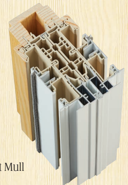
Continuous Head & Sill Mull Post
