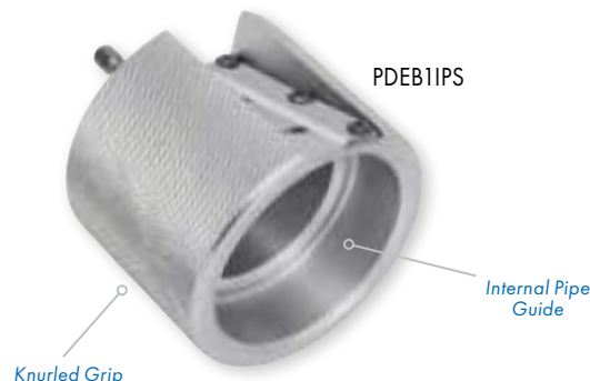
Knurled Grip
