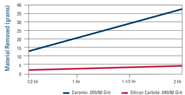
DEBURRING ACTION - BURR-RX (CG VS. SIC)
