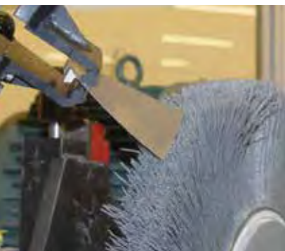
Deburring the tip of a turbine blade.
