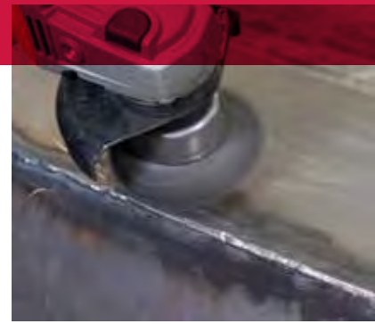
Knot wire cup brush removing heat discoloration.
