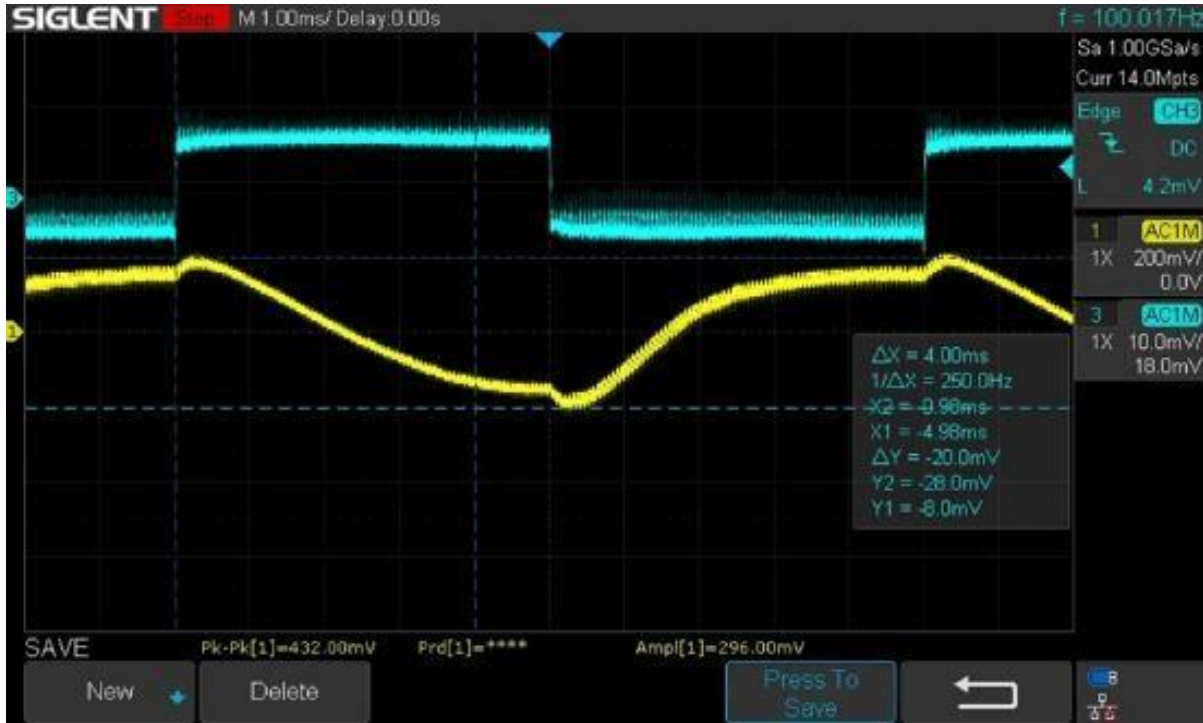
Figure 5 Typical Load Transient
