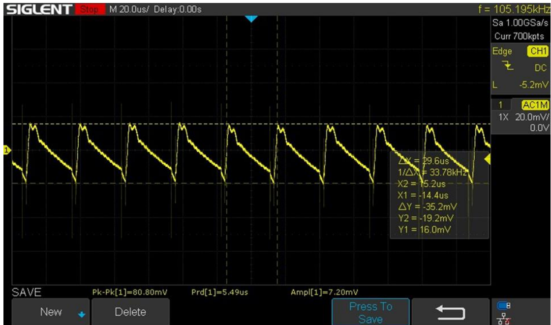
Figure 11 Ripple on V_{OUT2} Full Load
