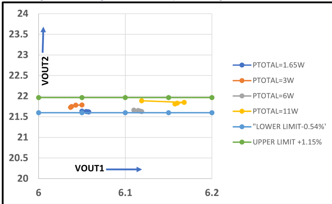
Figure 8 Cross Regulation with Total Power Output: Showing Tight Coupling
