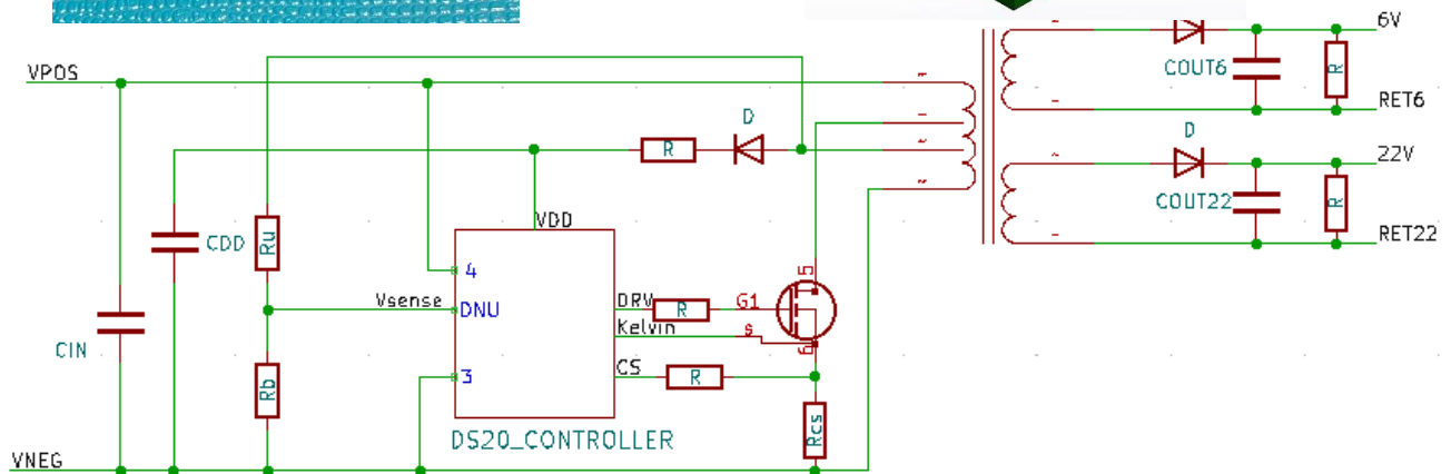
Figure 1 GMR10D000 Module Views and Schematic
