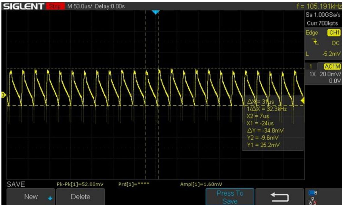
Figure 10 Ripple on Vout1 Full Load
