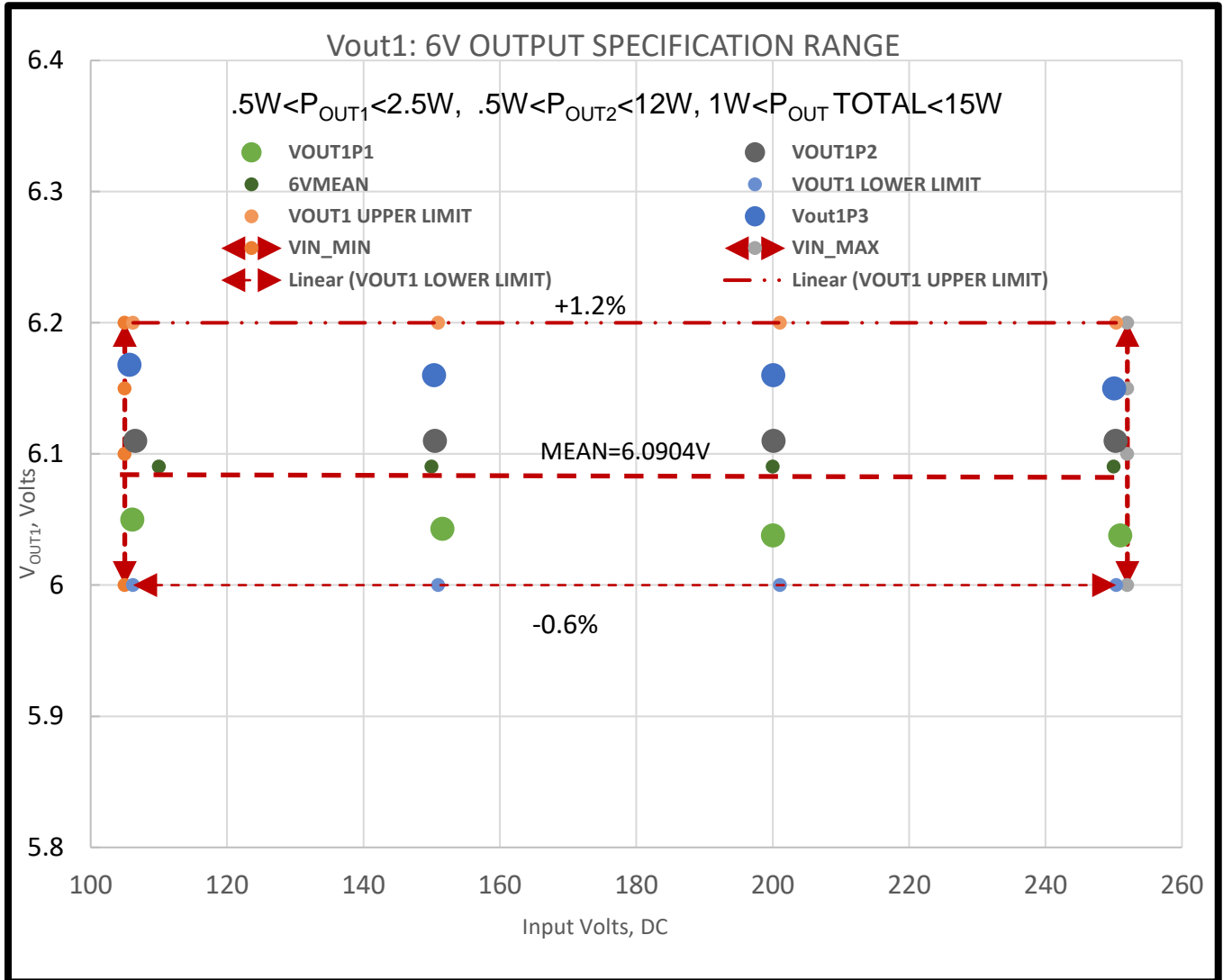
Figure 6 Load Regulation with DC Input: Showing Excellent Control
