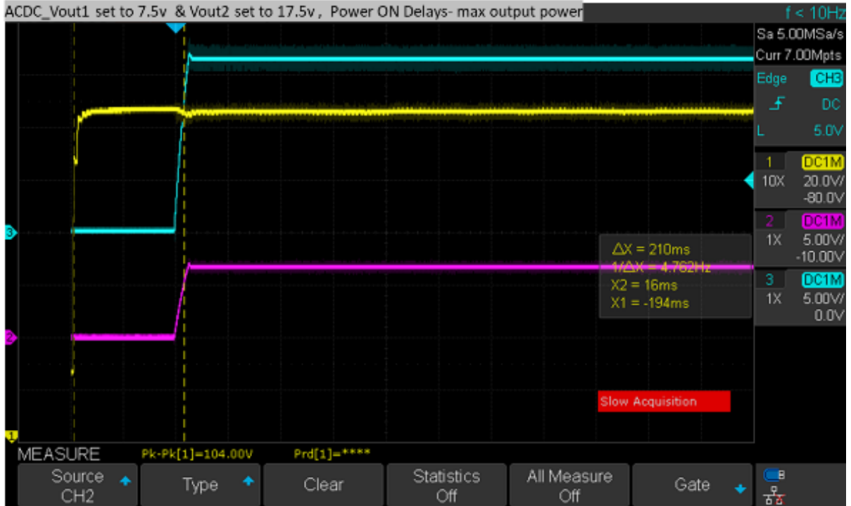
Figure 3 Reference 210 mS
