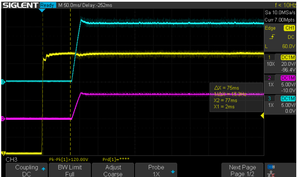
Figure 4 Turn ON Delay: Prototype Module Testing. Reference 75 mS
