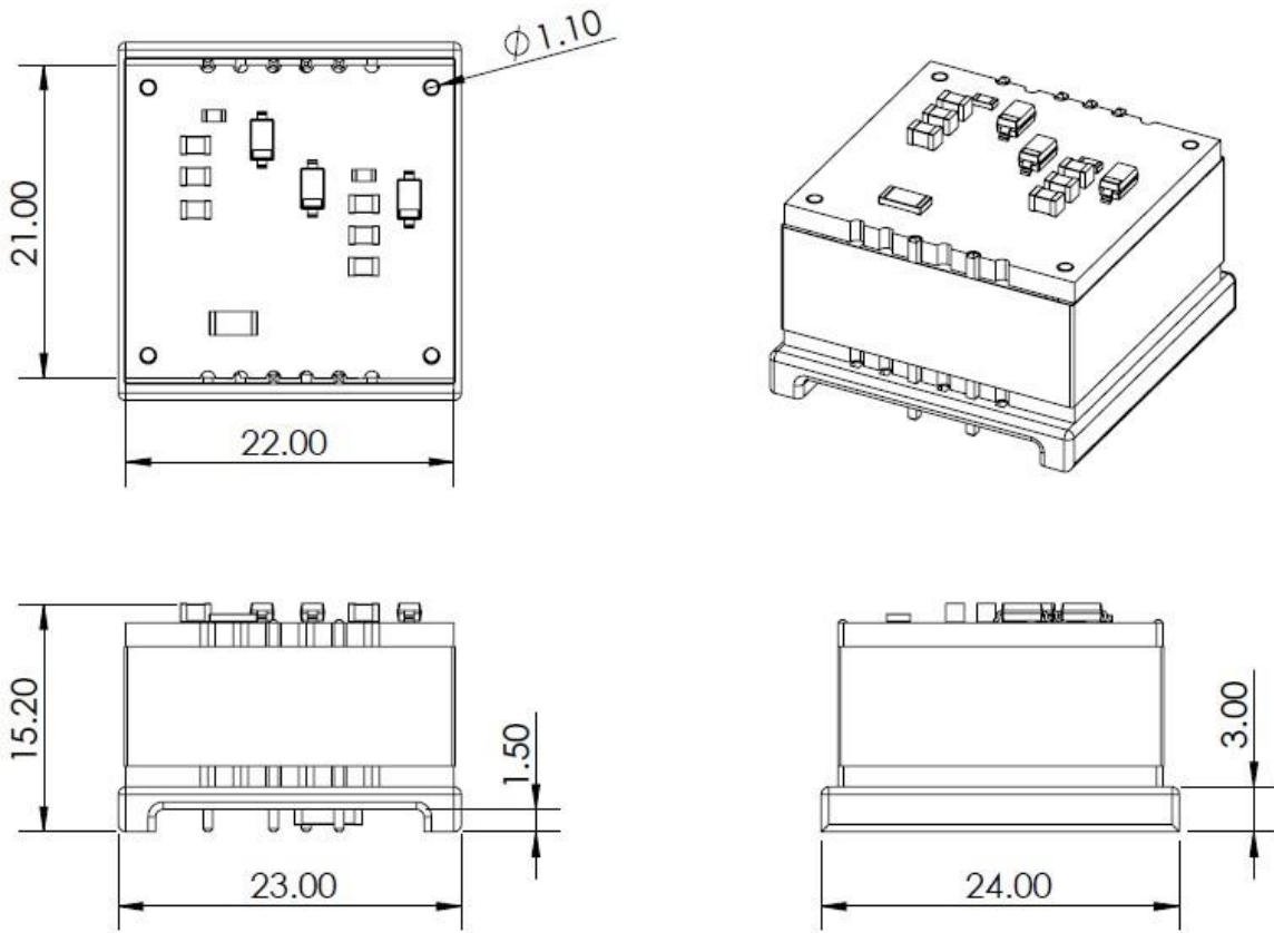
Figure 3 GMR10D000 Dimensions
