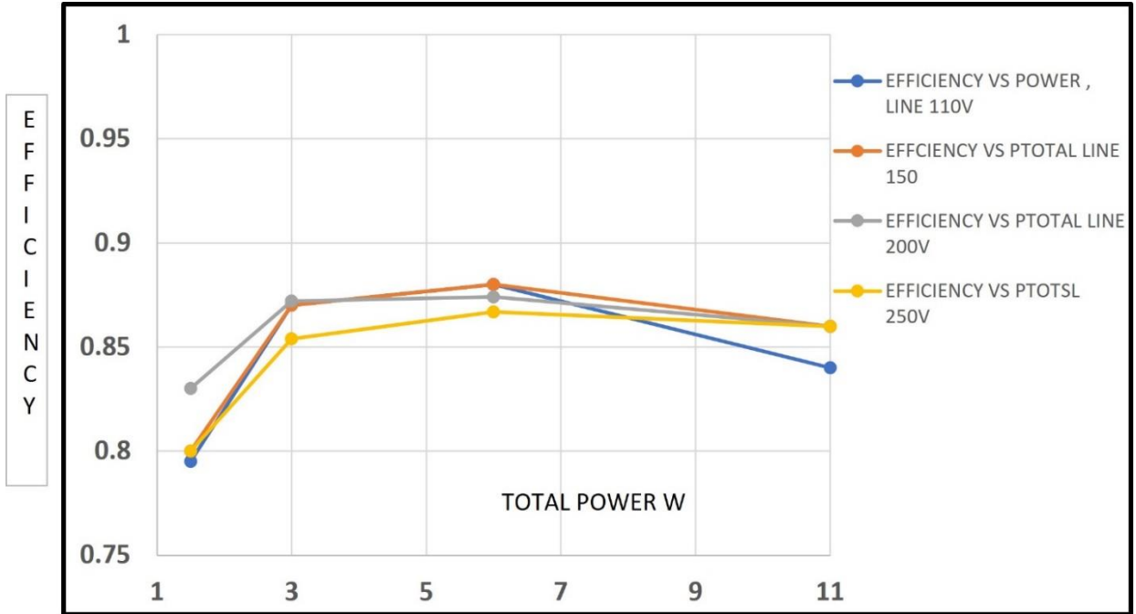
Figure 9 Efficiency with Total Power Output
