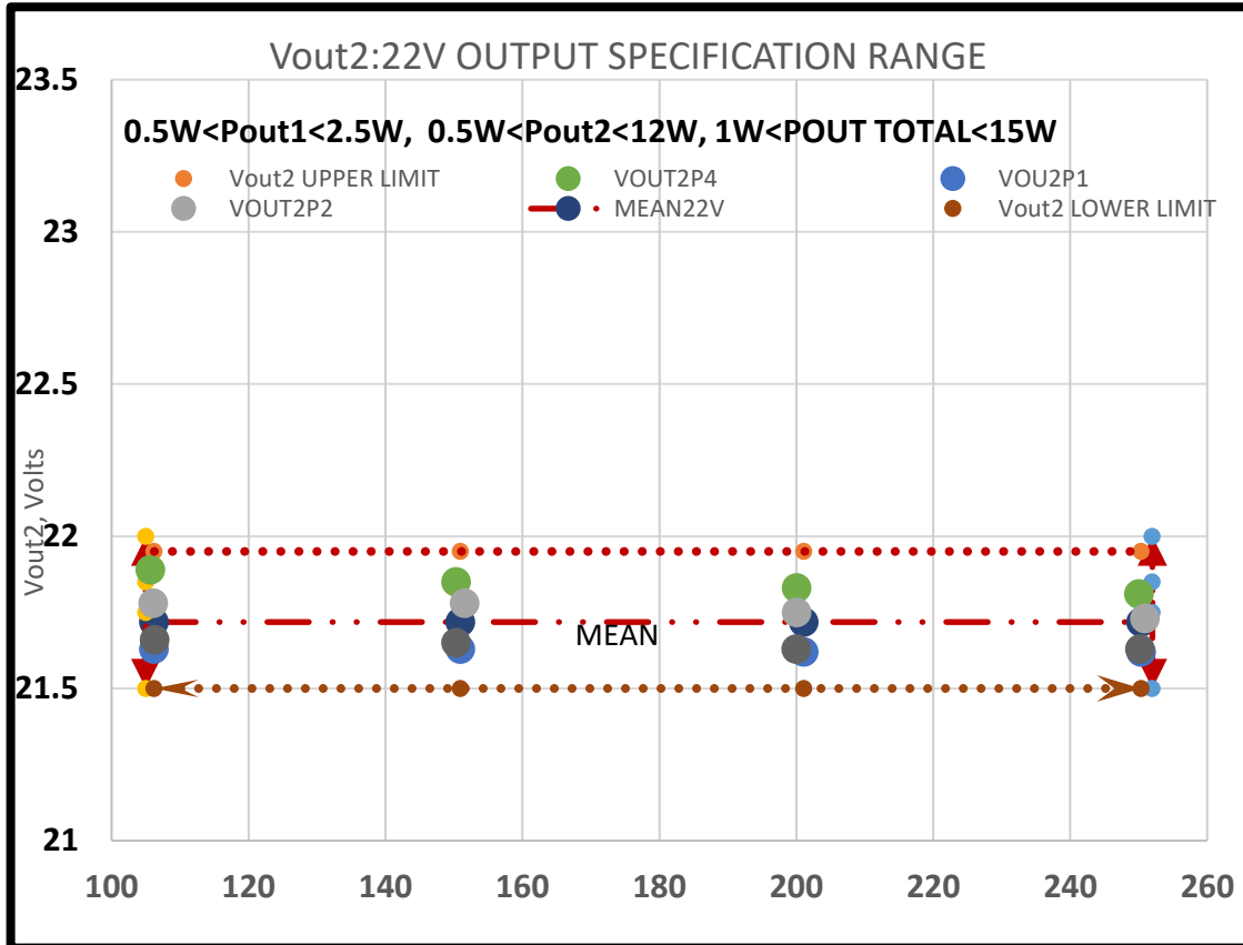
Figure 7 Load Regulation with DC Input: Showing Excellent Control 22V
