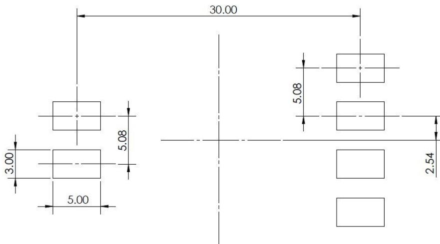
Figure 5 Through-hole Footprint
