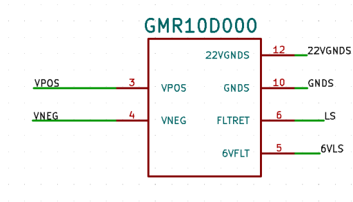
Figure 4 Pinout
