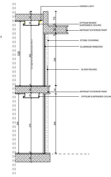
FACADE SECTION
