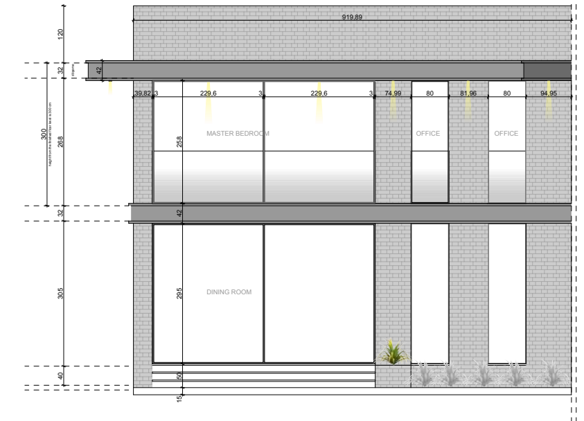
FACADE E
