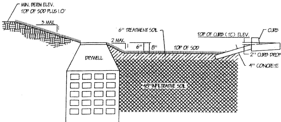
Grassy Drainage Swale - Typical Cross Section
