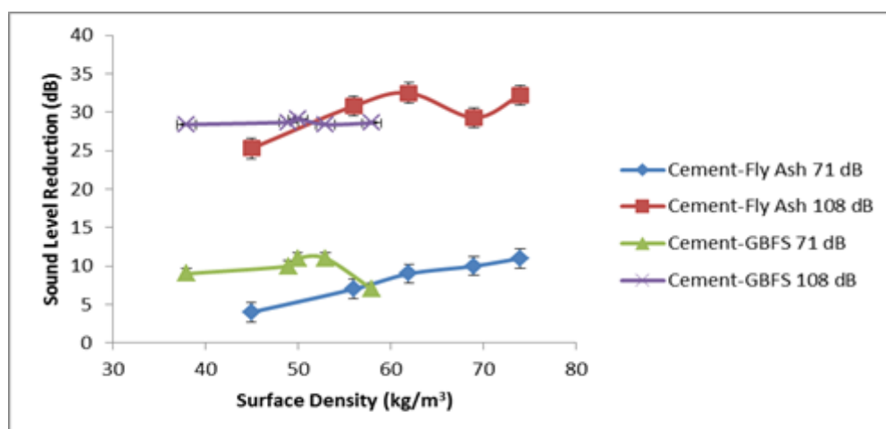
Figure-2: Relative sound level reduction vs. surface density
