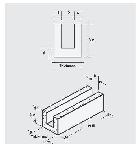
Fig. 3: Hebel® U-Block for horizontal reinforcement.
