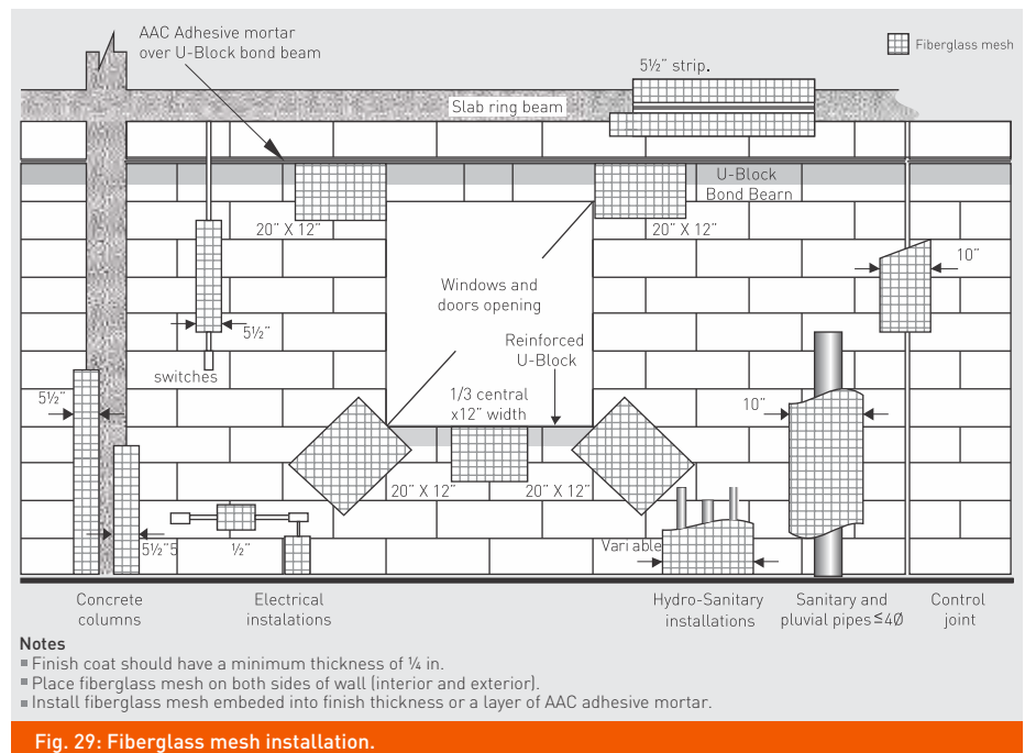
Fig. 29: Fiberglass mesh installation.
