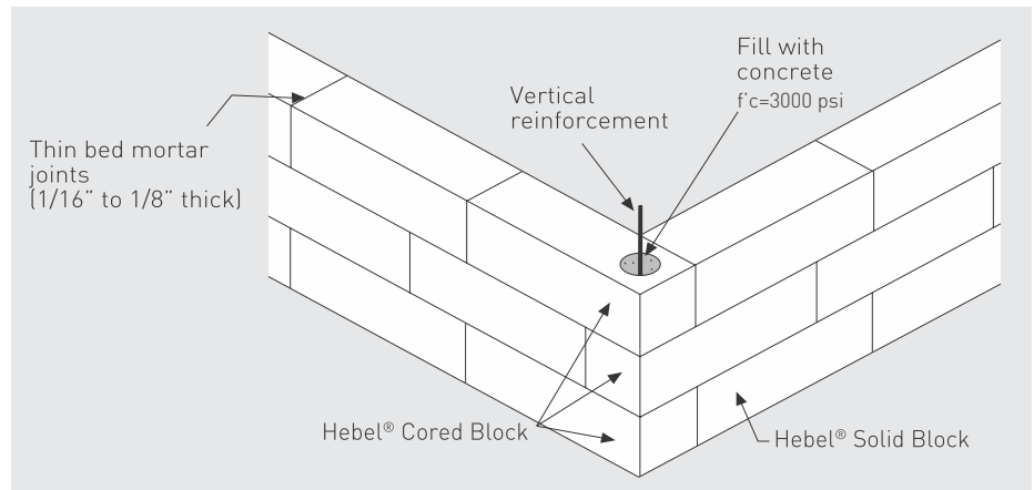
Fig. 11: Pilaster located at corner.
