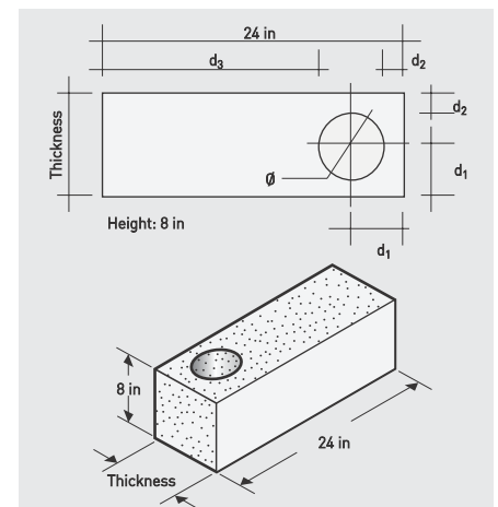
Fig. 2: Hebel® Cored Block for vertical reinforcement.
