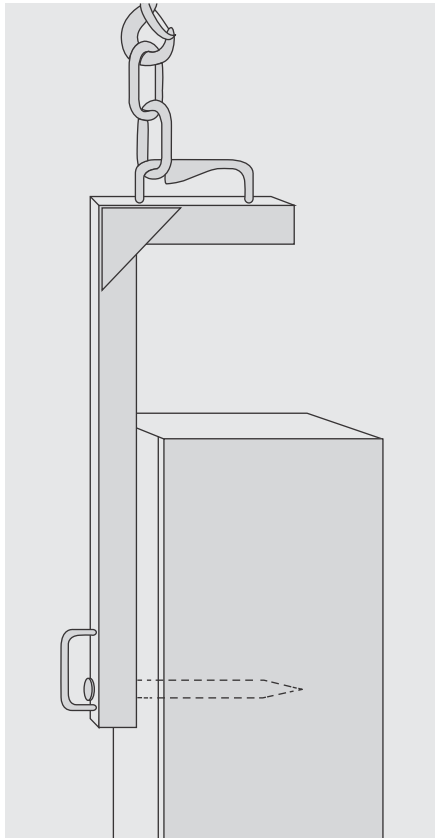
Fig.6b: Lifting hook (Hebel® vertical wall panels).
