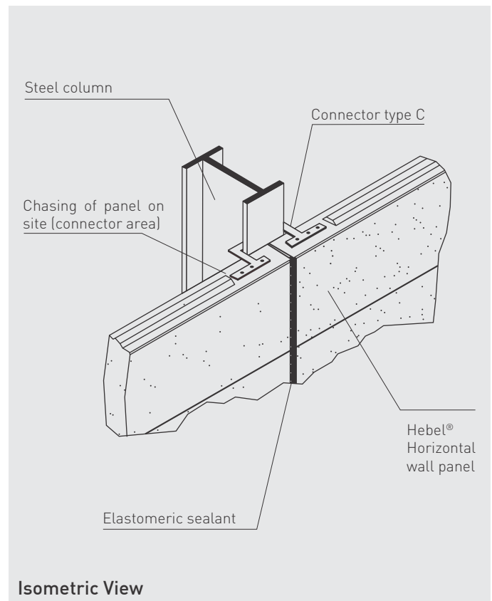
Fig. 3: Typical connection in Hebel® Horizontal Wall Panels using type "C" connector.
