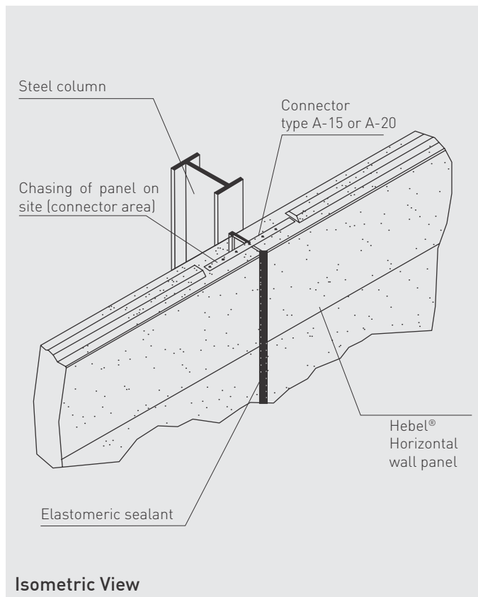
Fig. 2: Typical connection in Hebel® Horizontal Wall Panels using type "A" connector.
