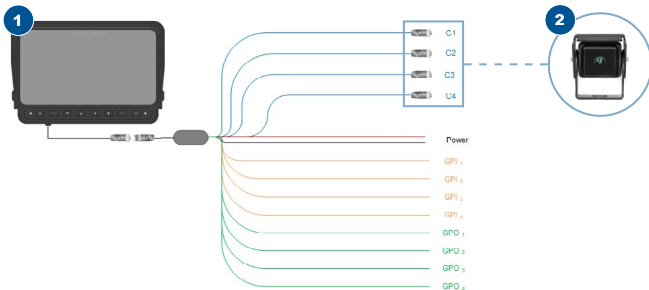
Heavy-Duty TVI AI Camera MCT3158-AI-4A
