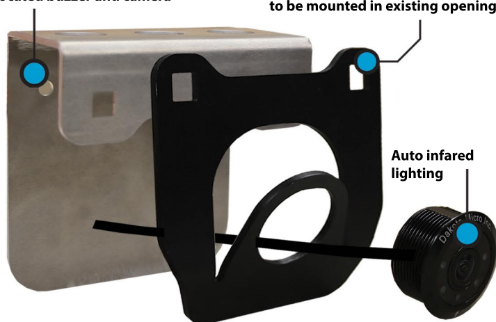
Custom heat shield for higher horse power Bobcats, which protects relocated buzzer and camera
