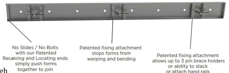
Super-Form Road Forms 6 months old
