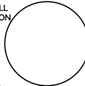
WAXING GIBBOUS
