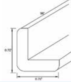
Outside Corner Molding - OCM8
