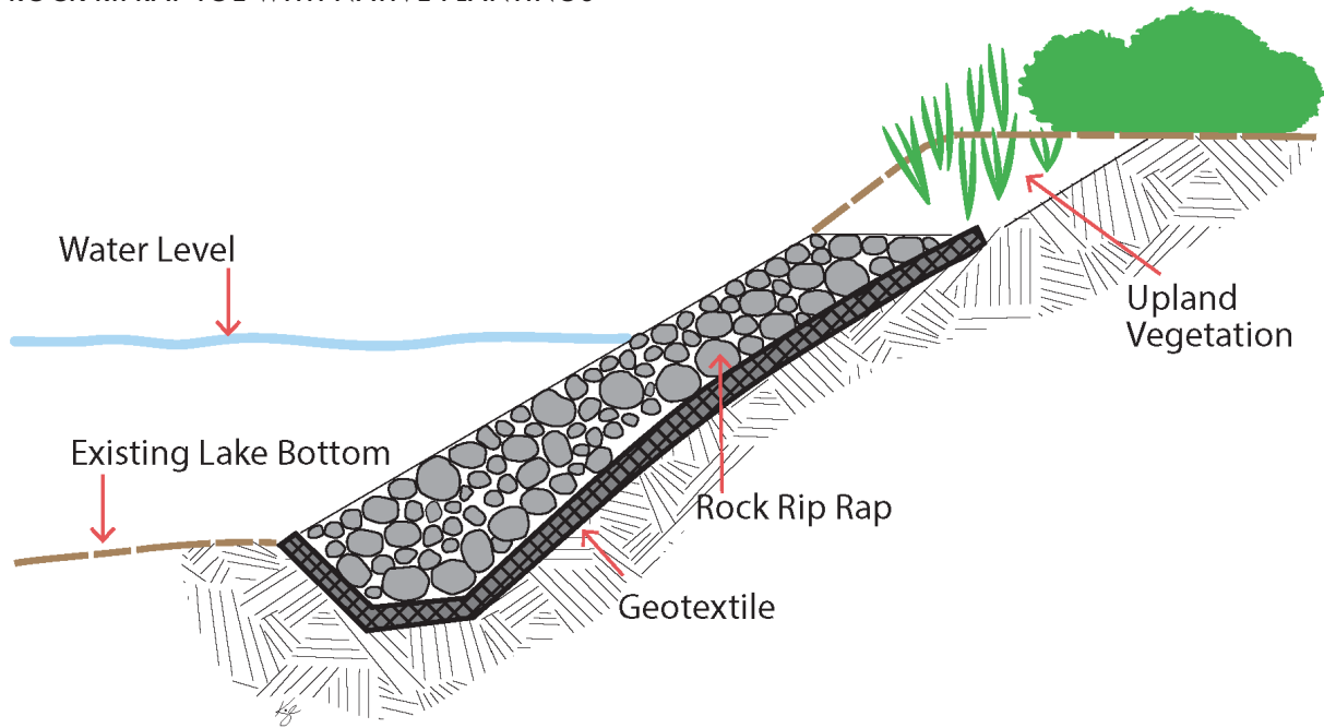
FIGURE 9: ROCK RIPRAP TOE WITH NATIVE PLANTINGS
