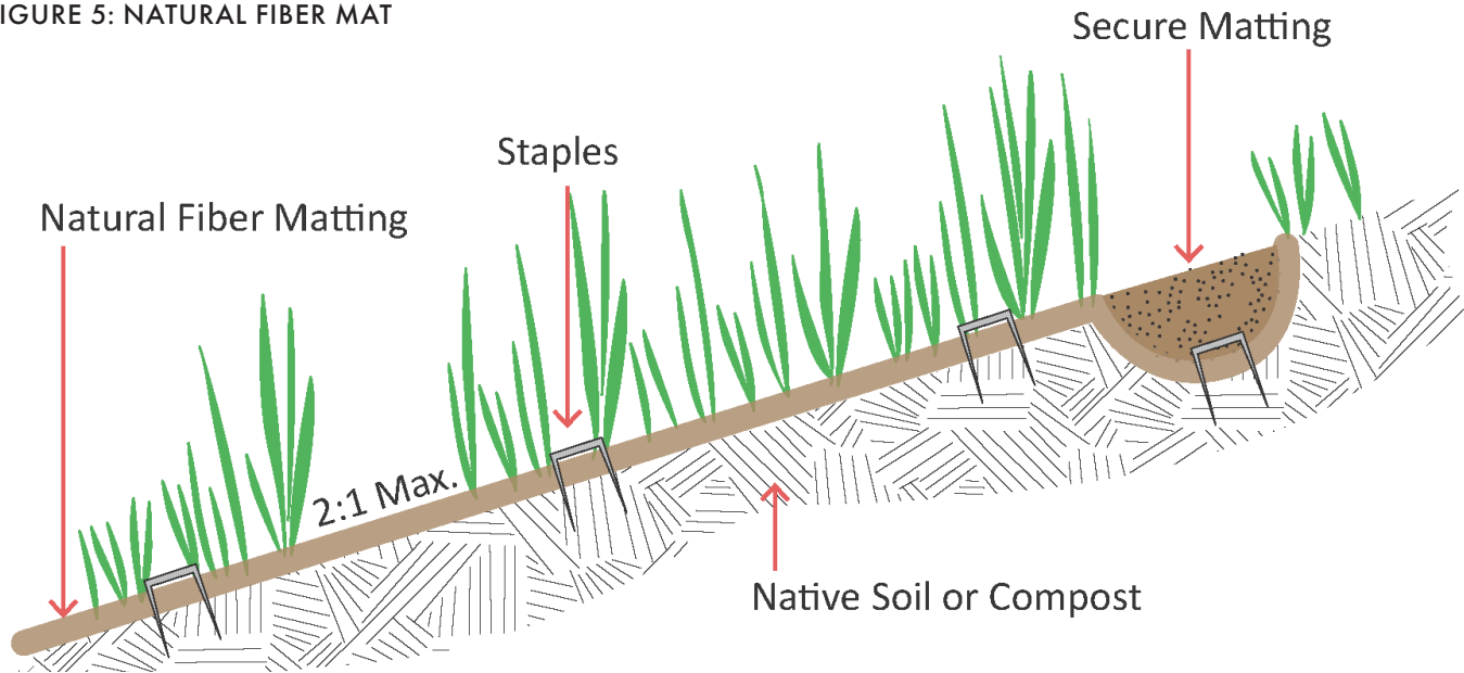
FIGURE 5: NATURAL FIBER MAT
