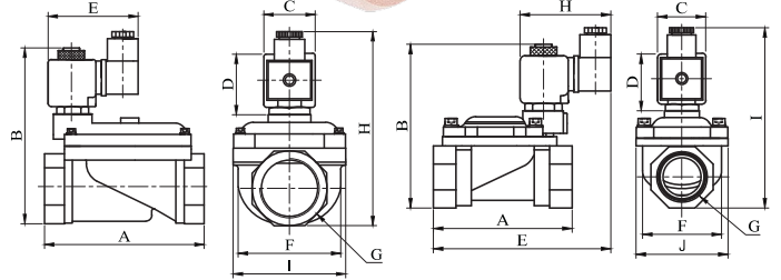
Dimensions (mm)
