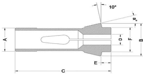
F-Type Collet (Angular face)
