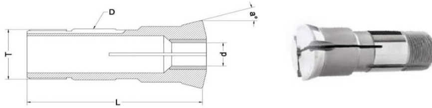
Guide Bush - Reinforced Shank Type
