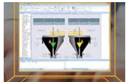
Software
