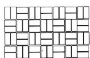
BASKETWEAVE Brick Size 92mm x 197mm
