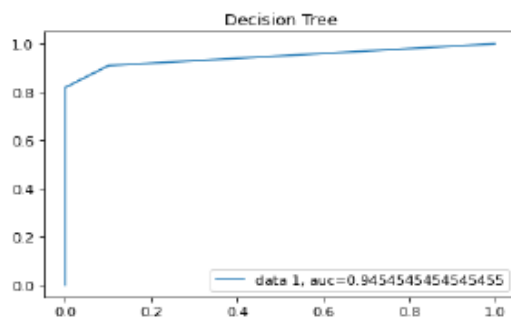
Figure 4: AUC value of Decision Tree
