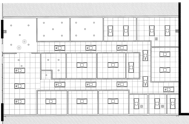
2 CEILING PLAN 3/16" = 1'-0"
