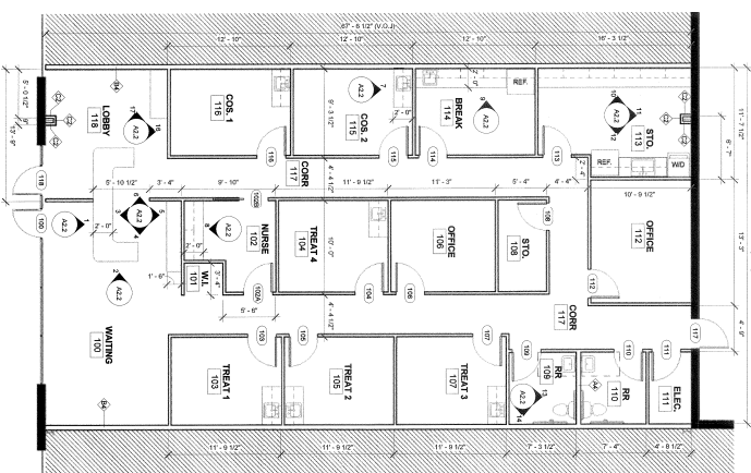
① FLOOR PLAN 3/16" = 1'-0"
