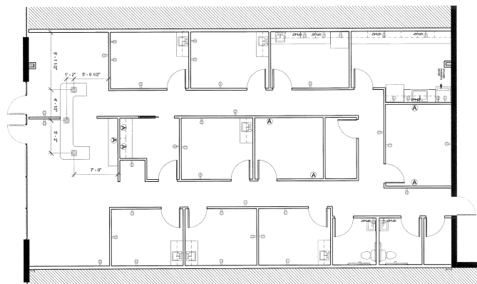
3 POWER PLAN 3'16" = 1'-0"
