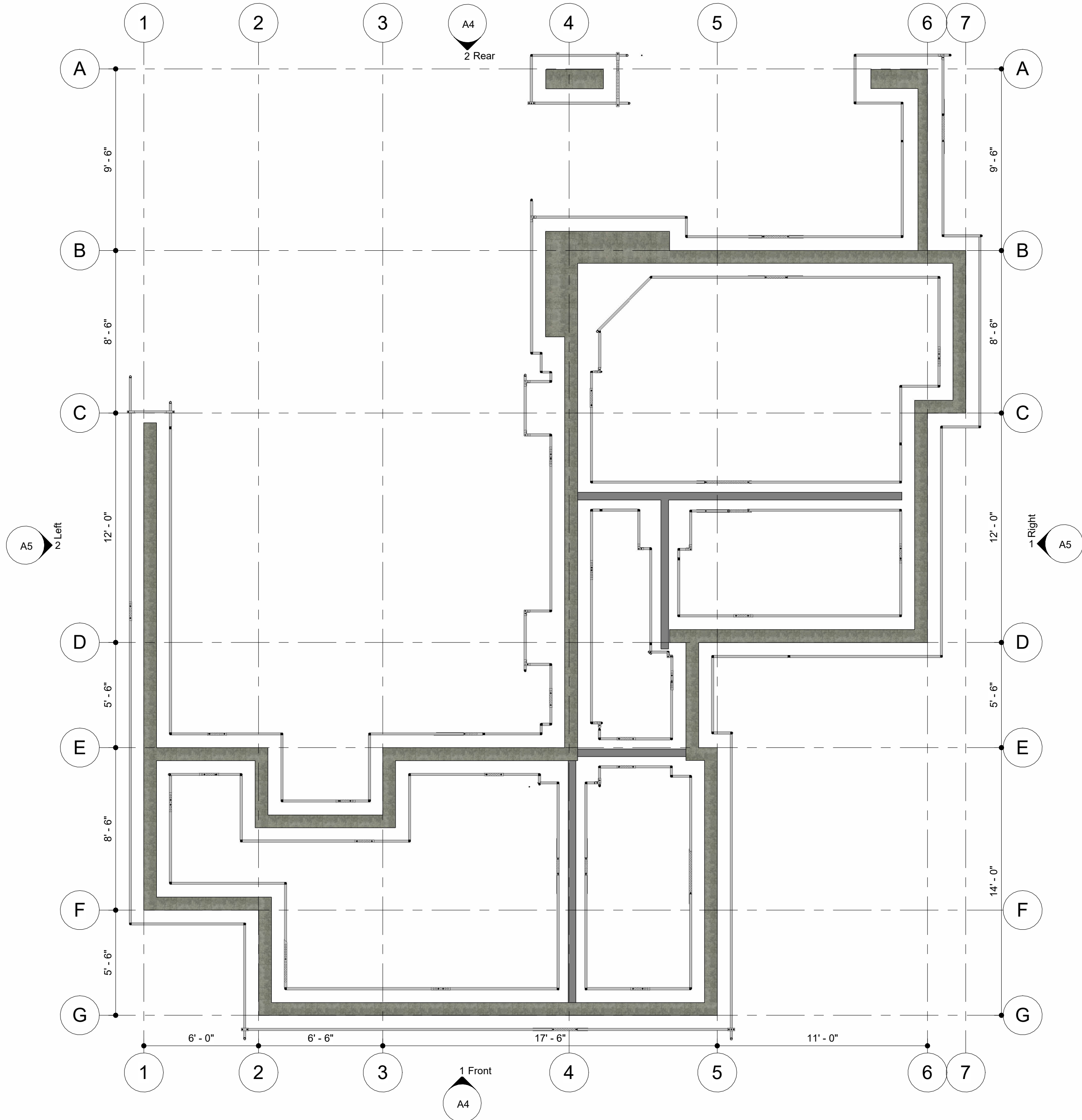
① BOFTG 1/4" = 1'-0"
