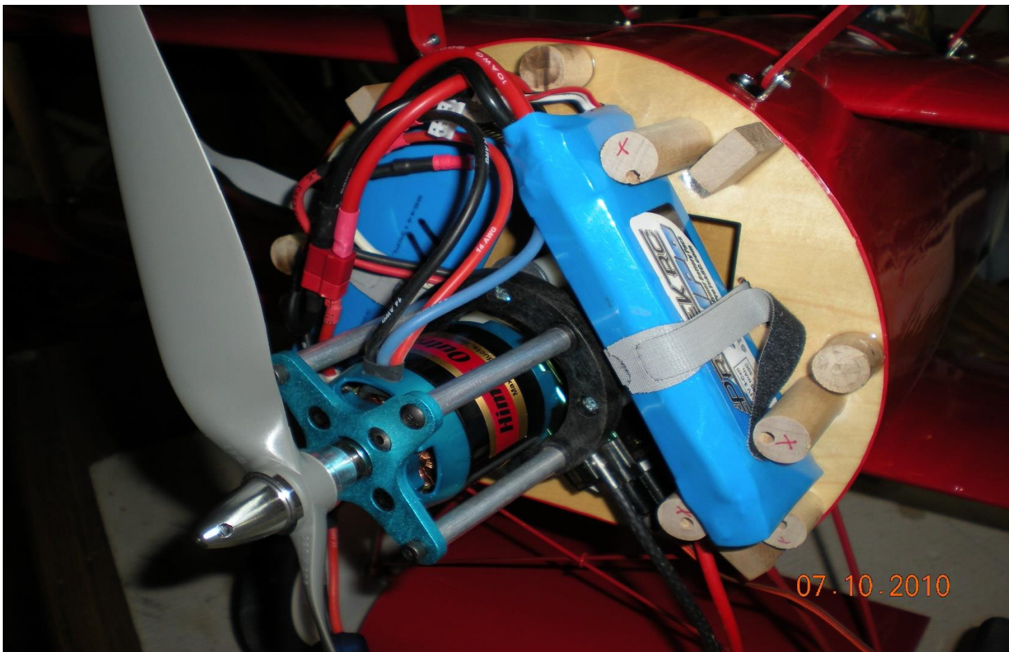
Typical electric setup when weight is needed up front
