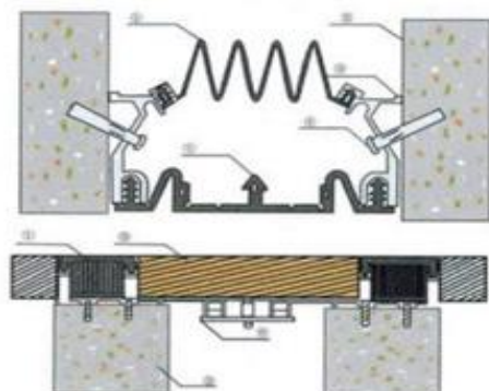
Building deformation joint rubber sealing strip
