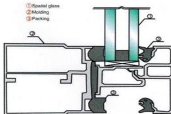
Rubber sealing strip for building curtain wall
