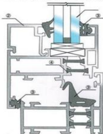
Rubber sealing strip for aluminum alloy energy saving door and window
