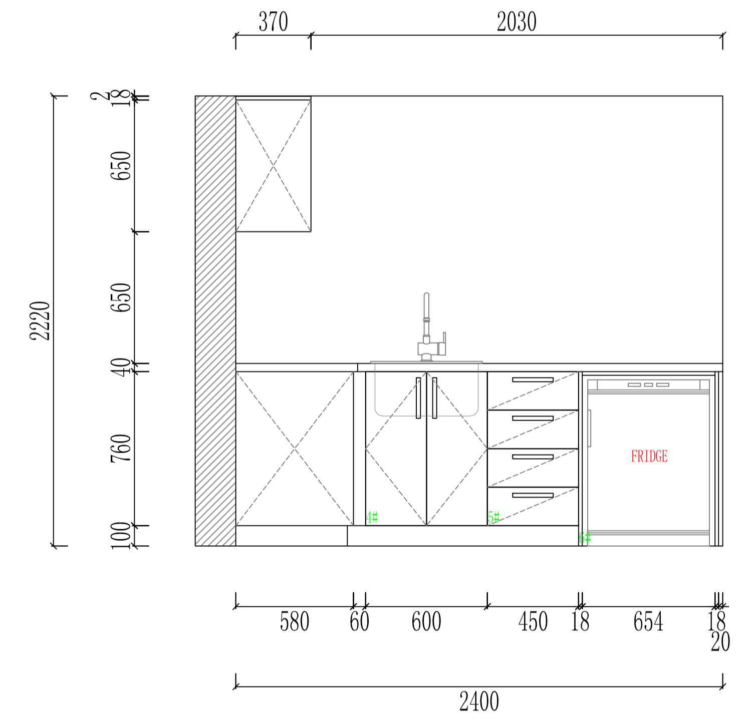
B VIEW
