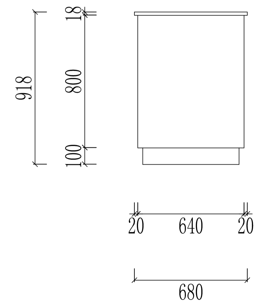
D VIEW
