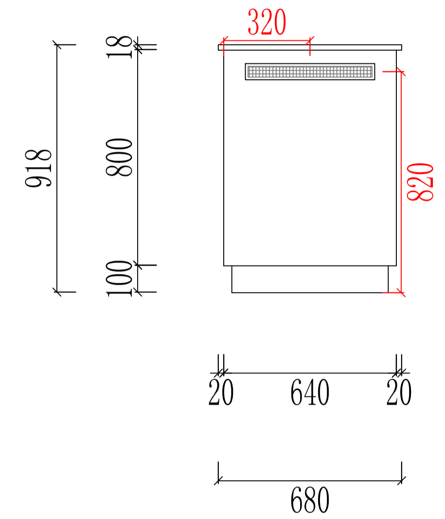
B VIEW
