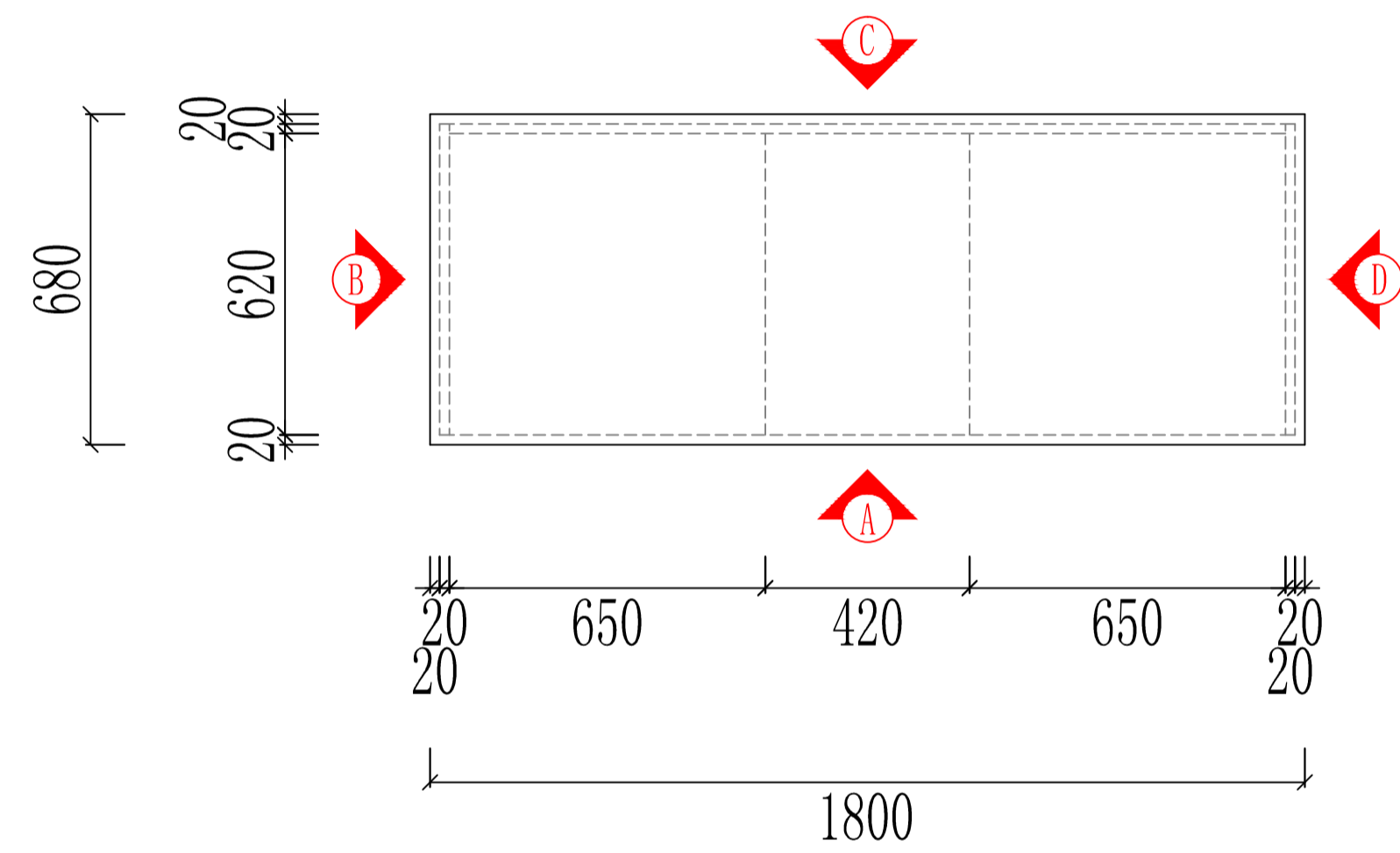
TOP VIEW
