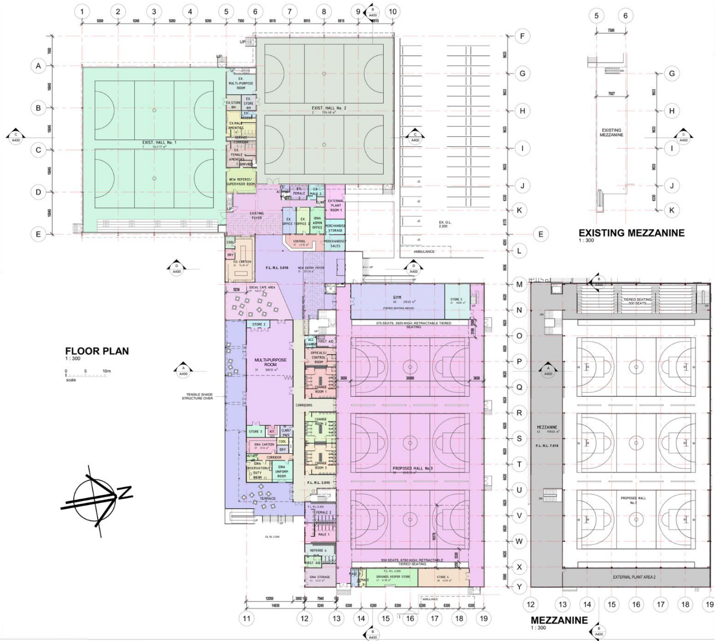
Figure 17. Floorplan of proposed ISS building
