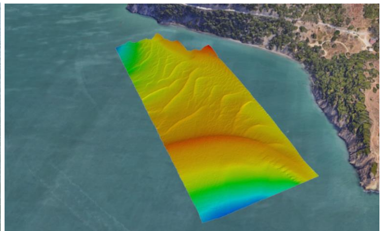
WAM-V 16 ASV hydrographic survey results
