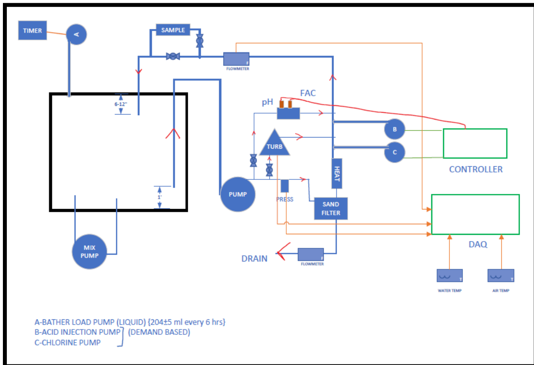
Figure 8- Test Setup
