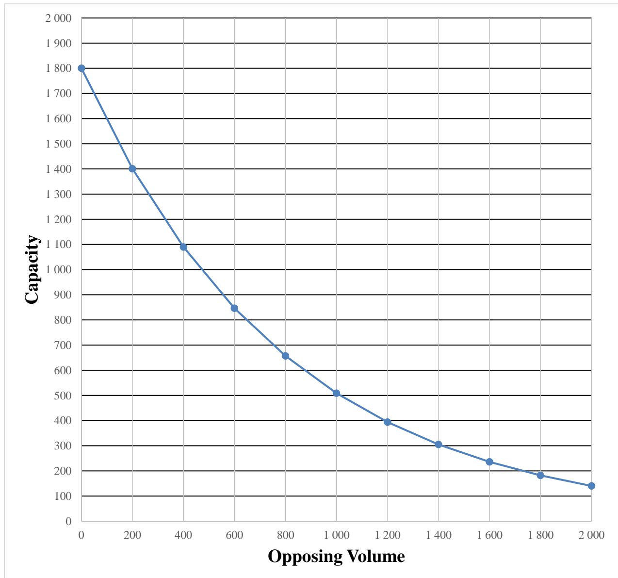
Figure 8: Typical Capacity Curve (“free” right turn)
