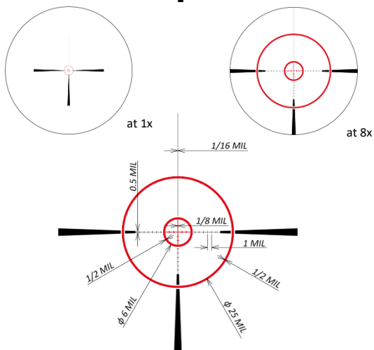
FMC-2 Reticle
