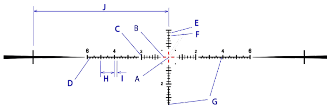
FML-3 & TR1 reticle subtensions
