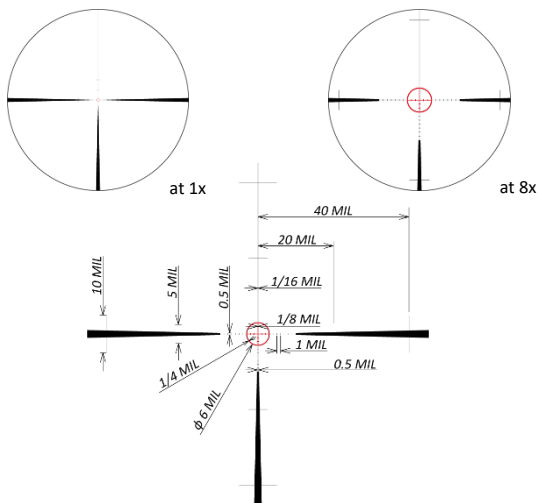
FMC-1 Reticle
