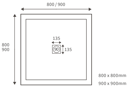
ULTRASLIM SQUARE TRAY
