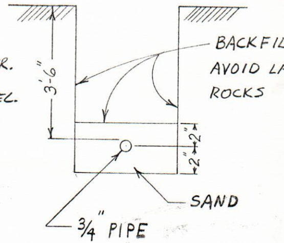
WATER SERVICE - BUILDING M TYPICAL TRENCH CROSS SECTIO
