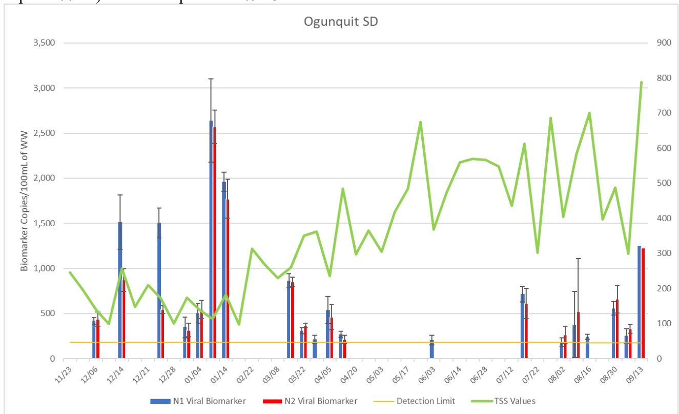
Figure 1: Temporal trends for Ogunquit SD overlain with TSS data.
