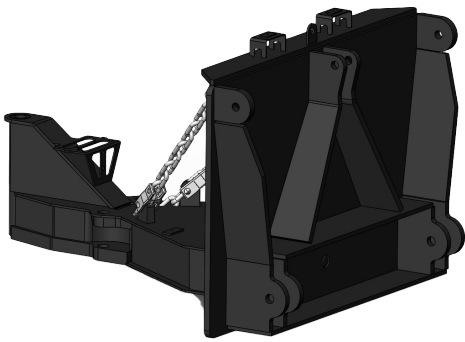
Typical Class 2 3/4 Point Hitch Mount
