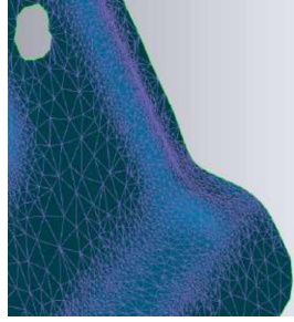
Figure 28 – Optimized Mesh
