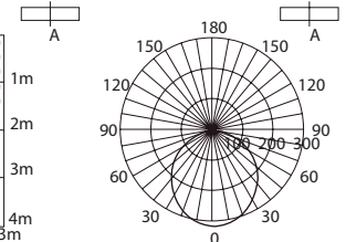
Candlepower Distribution
