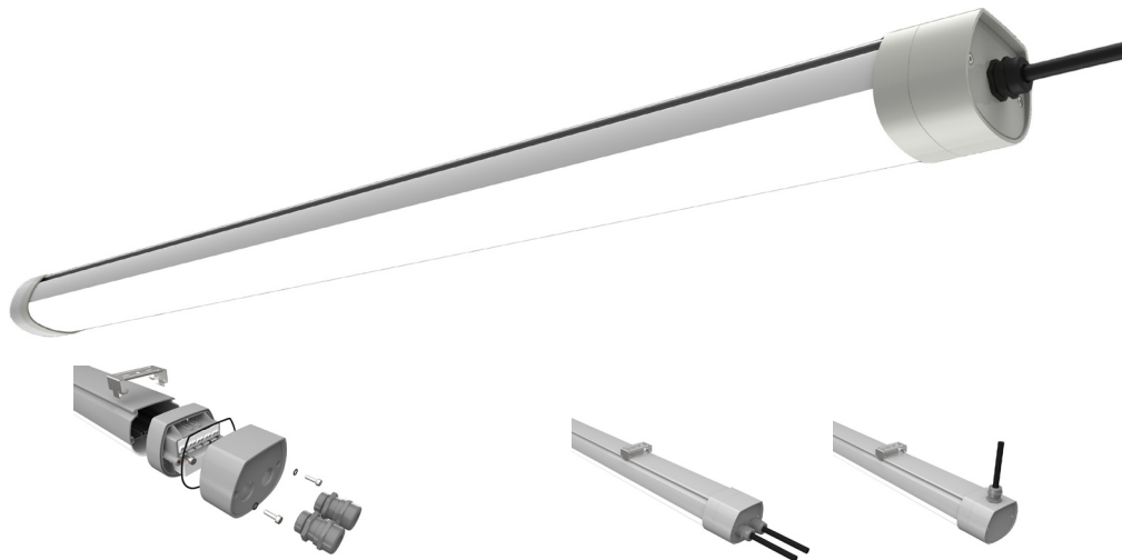
Integral - termination bulkhead
