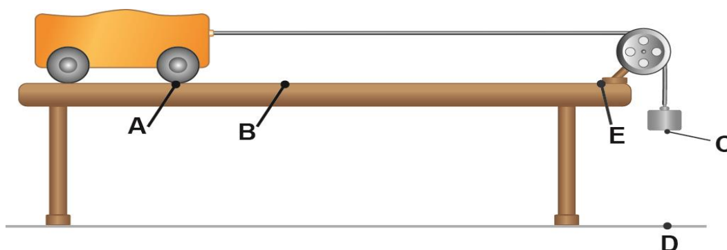
Figure-1. Practical set up to demonstrate the effect of constant force
