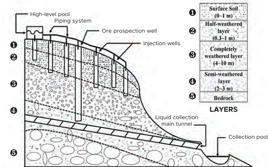
Figure 4.6: Schematic diagram of in-situ leaching mining set-up (Vahidi, Navarro & Zhao, 2016)
