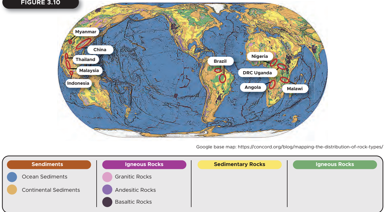
Figure 3.10: Composite geology map of the world showing tin granite distribution (Pallant, 2022)
