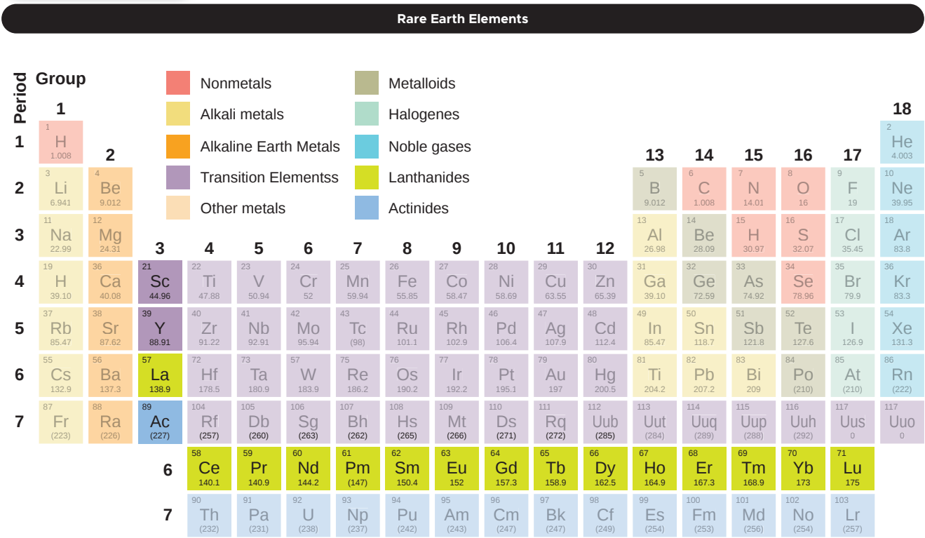
Figure 3.1: The periodic table showing 15 elements of the lanthanide series and two elements in Group 3 (all 17 elements are considered critical elements) (Rare Element Resources, 2023)
